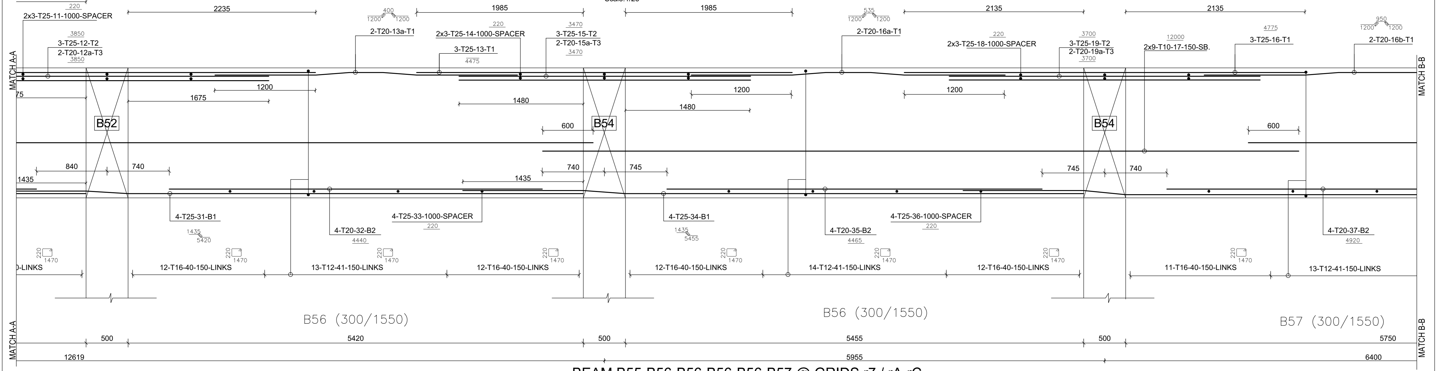
BEAM B55-B56-B56-B56-B56-B57 @ GRIDS rA-rC
