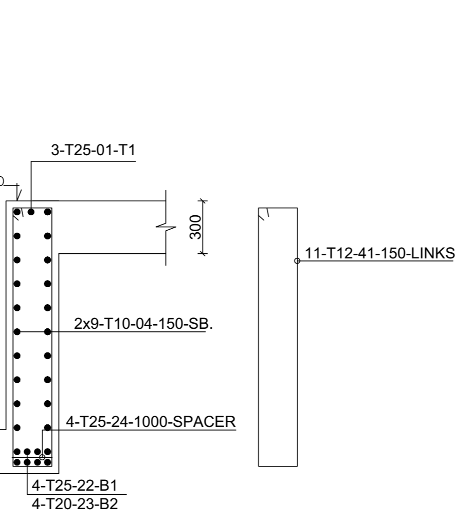
SECTION 01-01
