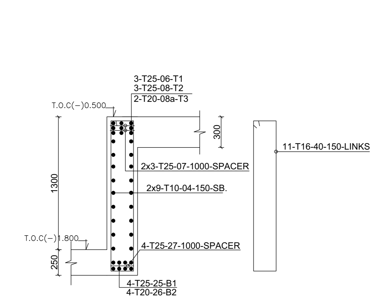
SECTION 02-02
